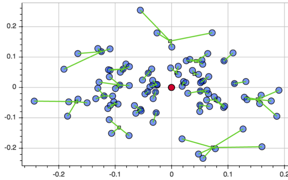
Figure 3: Regularized geometric k -median for carpool meetup problem. 26 ride share groups from 100 users.
